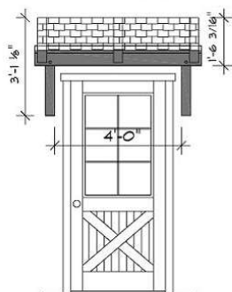
4' Eyebrow Roof "K" $1,500 (for a 3' door)
