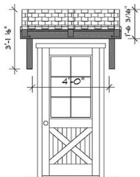
4' Eyebrow Roof "K" $1,250 (for a 3' door)
