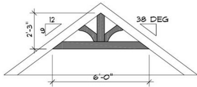
Straight Accent Truss "F" $600
