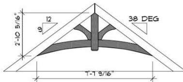
Arch Accent Truss "E" $700
