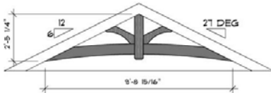
Arch Accent Truss "C" $700
