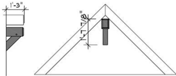
Corbel "B" $250 (no vents when corbels are installed)
