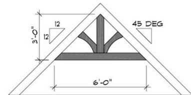
Straight Accent Truss "H" $1,300
